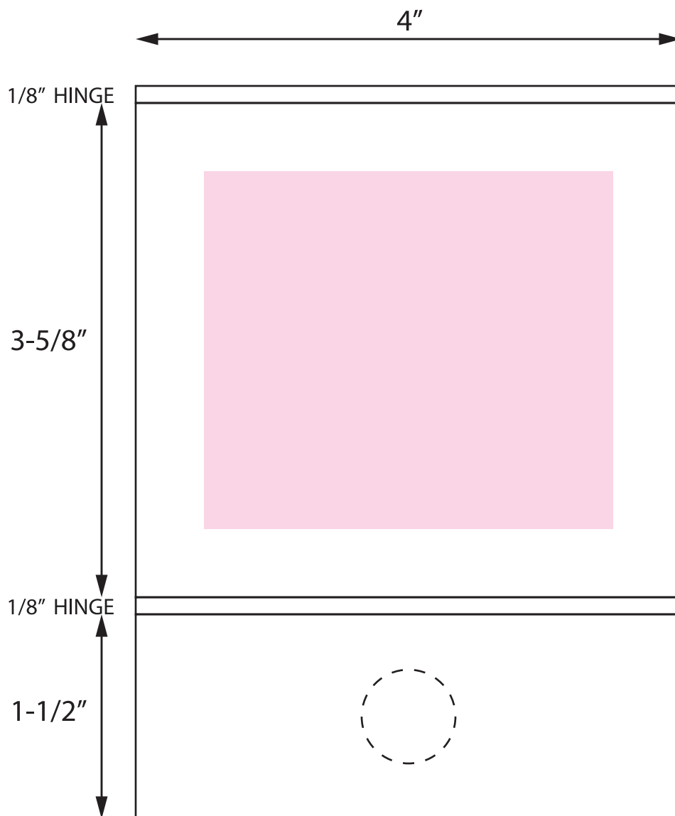
EXTERIOR DIMENSIONS
